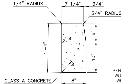
CURB DETAIL
